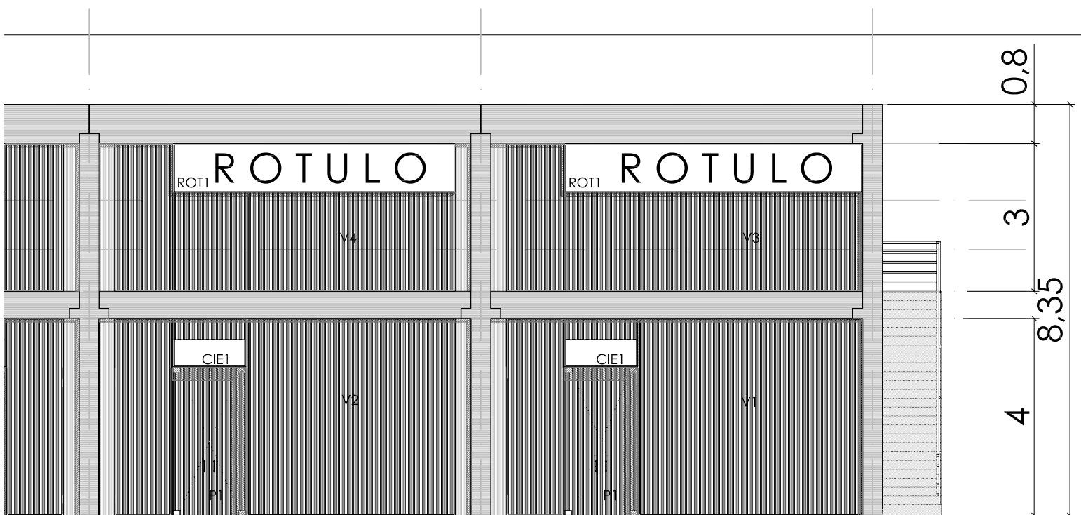
ALZADO PRINCIPAL
